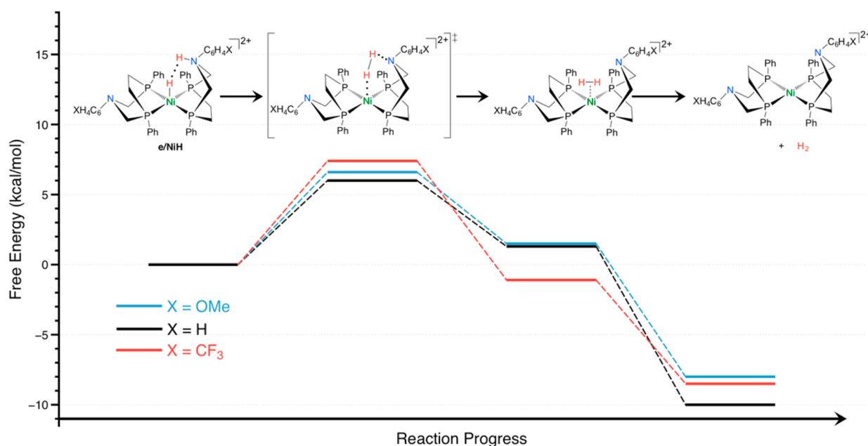
Figure 11. Lowest free energy \text{H}_2 elimination pathway for 5-OMe , 5-H , and 5-CF 3 .
