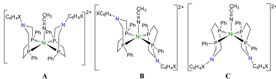
Figure 2. Proposed isomers of 5 in \text{CH}_3\text{CN} .
