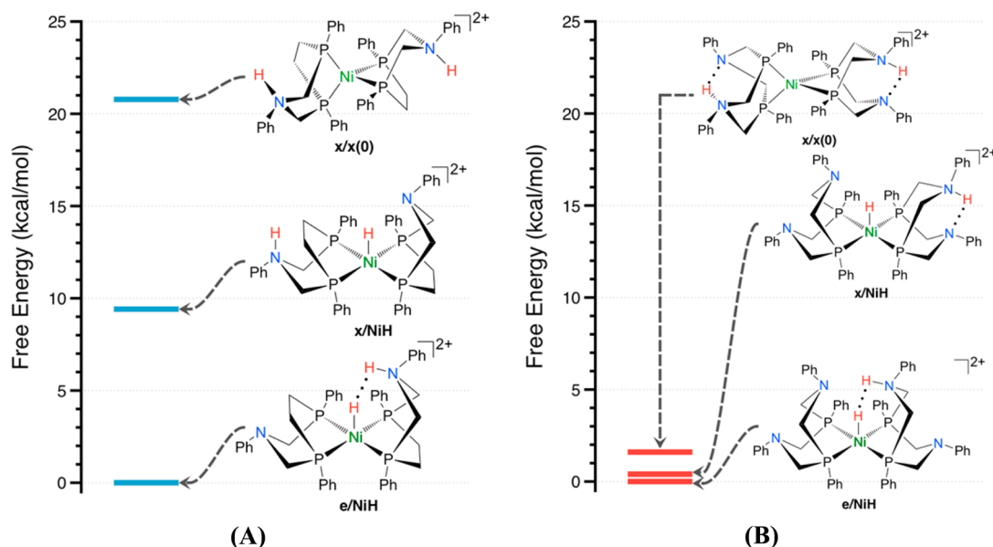
Figure 10. Ranking of the lowest free energy isomers of the doubly protonated complexes of (A) [\text{HNi}(\text{7P}^{\text{Ph}}_2\text{N}^{\text{C6H4X}}\text{H})(\text{7P}^{\text{Ph}}_2\text{N}^{\text{C6H4X}})]^{2+} / [\text{Ni}(\text{7P}^{\text{Ph}}_2\text{N}^{\text{Ph}}_2\text{H})_2]^{2+} and (B) [\text{HNi}(\text{P}^{\text{Ph}}_2\text{N}^{\text{Ph}}_2\text{H})(\text{P}^{\text{Ph}}_2\text{N}^{\text{Ph}}_2)]^{2+} / [\text{Ni}(\text{P}^{\text{Ph}}_2\text{N}^{\text{Ph}}_2\text{H})_2]^{2+} .
