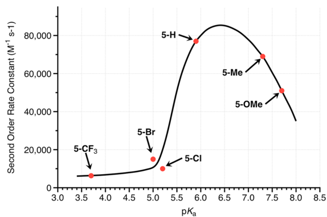
Figure 13. Graph of calculated \text{p}K_a values of the endo protonated, \mathbf{e(I)} [\text{Ni(7P}^{\text{Ph}}_2\text{N}^{\text{C6H4X}}\text{H})(7P}^{\text{Ph}}_2\text{N}^{\text{C6H4X}})_2]^{2+} complexes versus their second-order rate constants for hydrogen production. Black line between data points was added to illustrate the trend.
