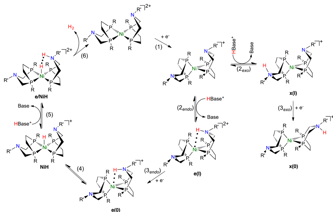
Figure 8. Proposed mechanism for catalytic H 2 formation.
