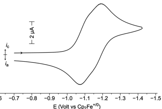
Figure 3. Cyclic voltammogram of 1.0 mM [\text{Ni}(7\text{P}^{\text{Ph}}_2\text{N}^{\text{C6H4OMe}})_2]^{2+} , 5-OMe , in 0.10 M [\text{Bu}_4\text{N}][\text{PF}_6]/\text{CH}_3\text{CN} . Conditions: 1 mm glassy carbon working electrode; scan rate 0.1 V/s at 25^\circ\text{C} .
